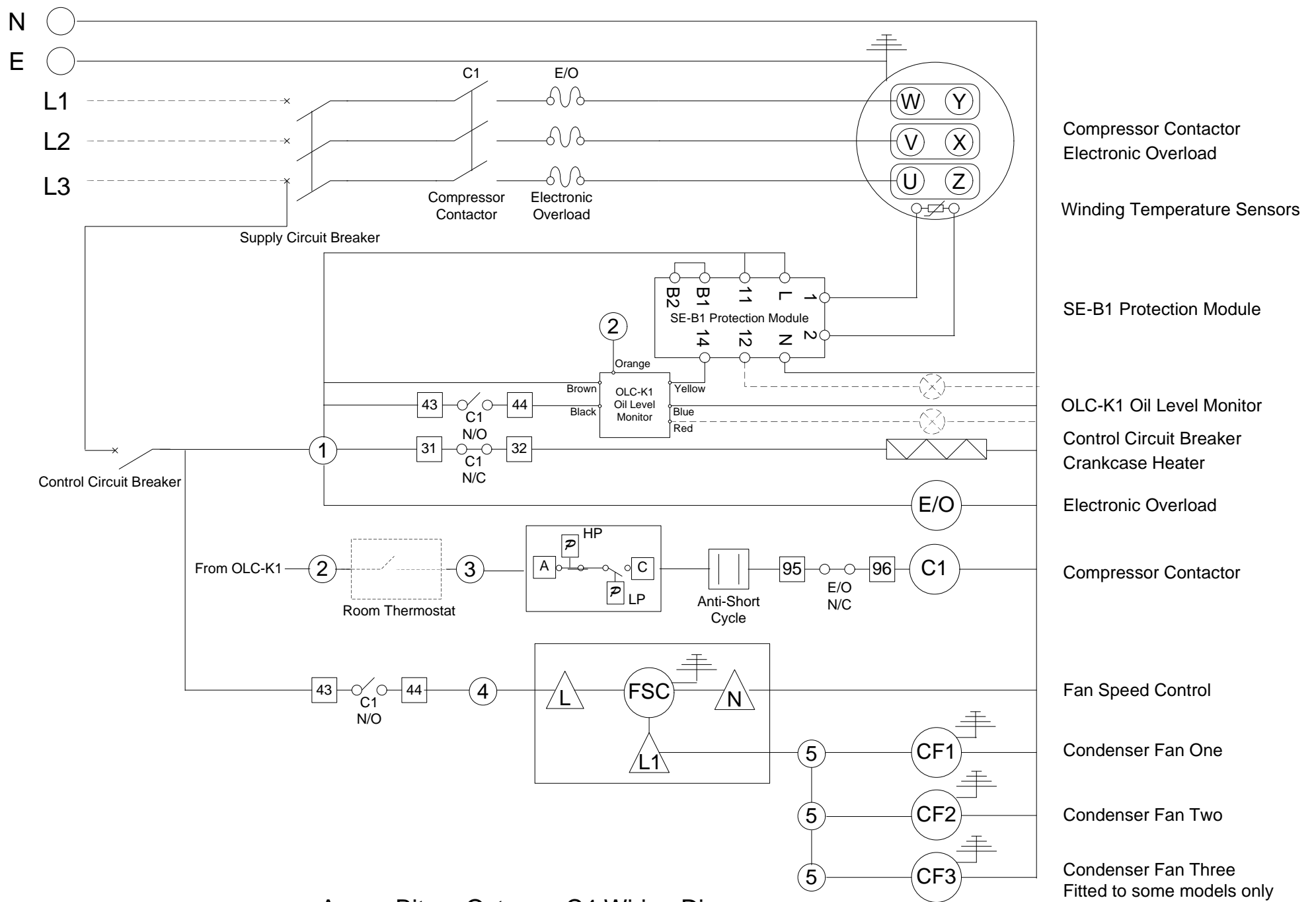
Acpac Bitzer Octagon C4 Wiring Diagram
