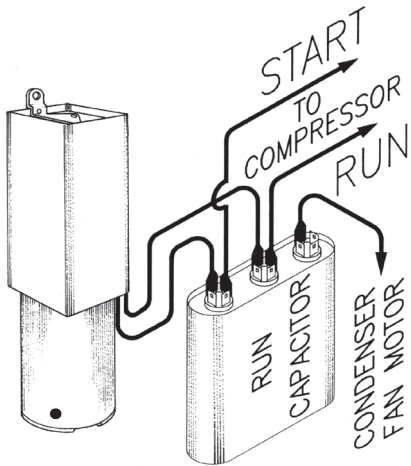
DUAL CAPACITOR
