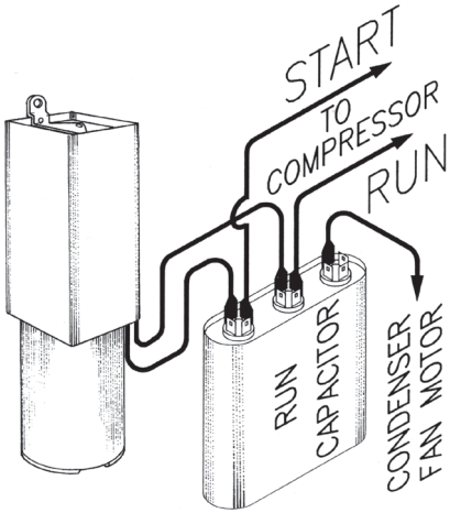
DUAL CAPACITOR
