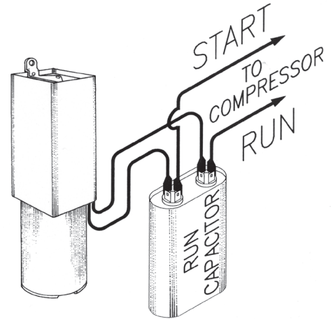
STANDARD CONNECTION
