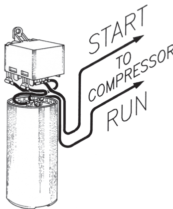
CSIR COMPRESSOR
